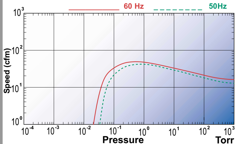
iL70 Pumping Speed Curve
