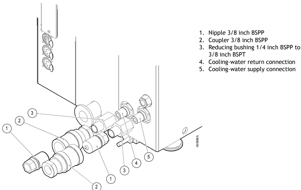
Figure 11 - Installing 3/8" quick connect fittings (provided)
