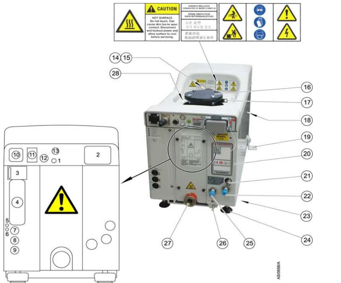
Figure 2 - The controls/connectors
