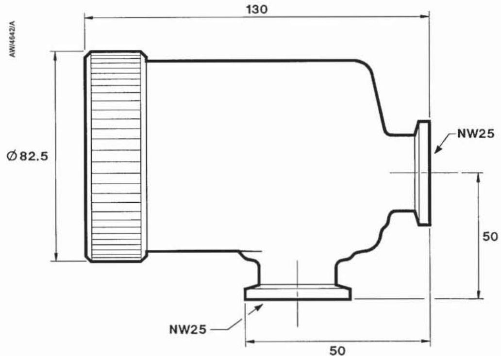
Figure 2 - Dimensions (mm)
