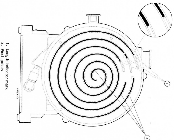
Figure 4 - Tip seal length
