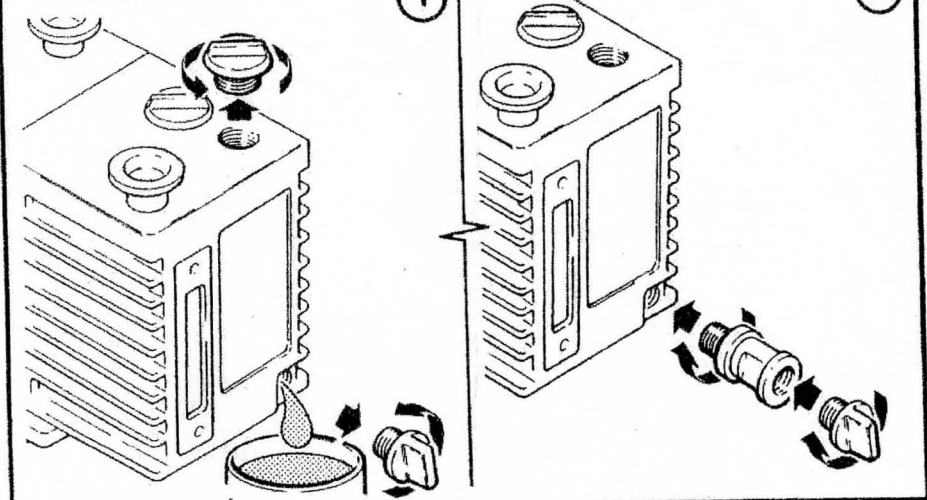
Oil Drain Extension A505-03-000
