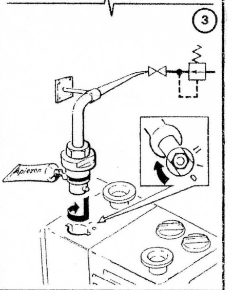
Exhaust Nozzle A505-09-000
