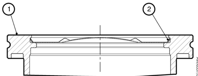
Figure 26 - ISDX inlet-screen
