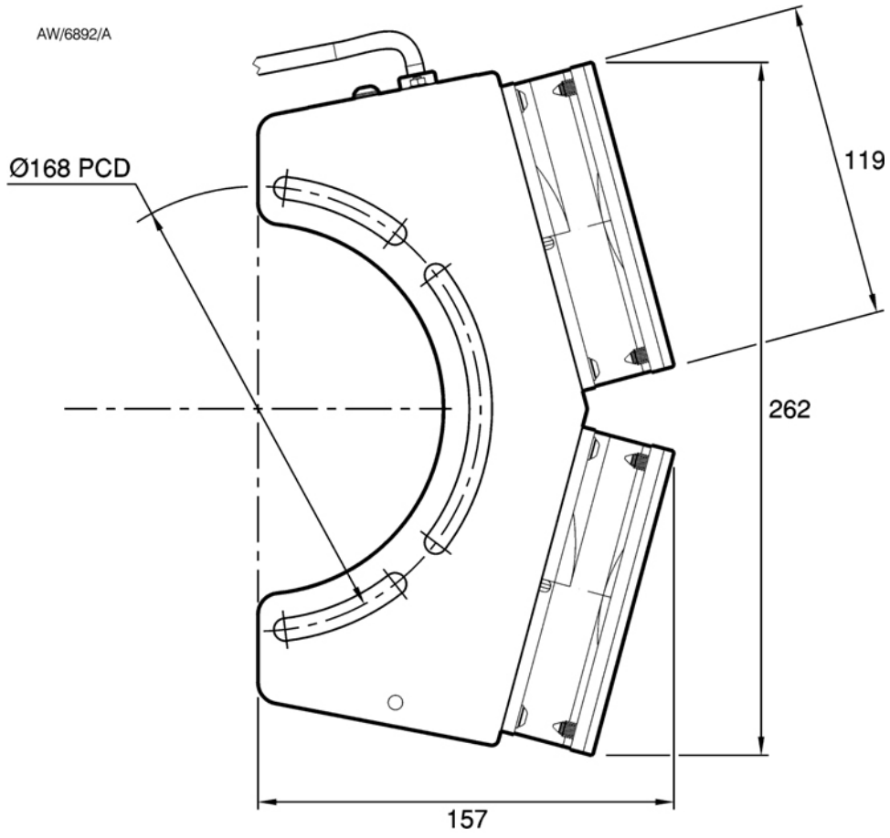
Figure 19 - ACX555 air-cooler dimensions (mm)
