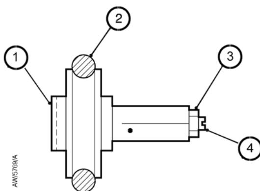
Figure 28 - PRX10 purge-restrictor
