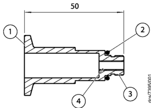
Figure 30 - Extended vent-port adaptor
