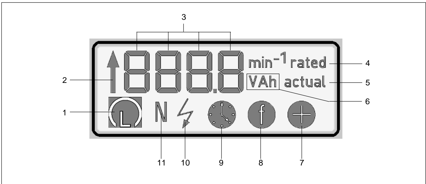
Fig. 5 Operating panel of the frequency converter
