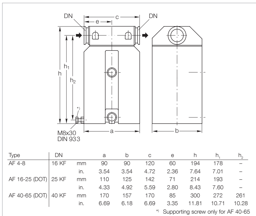
Dimensional drawing for the AF exhaust filters
