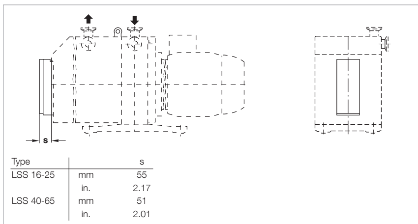
Dimensional drawing for the LSS (mounted on a TRIVAC BCS)
