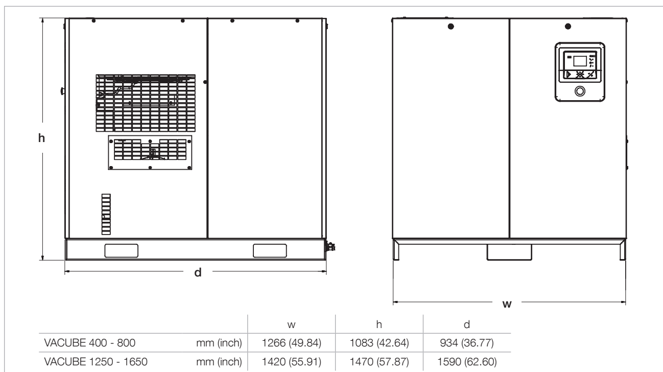
Dimensional drawing VACUBE
